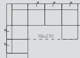
NAR.2BF/H/3W/1OT 245x338x174 | 174 | 85-99
