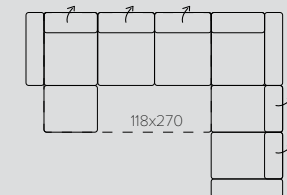
NAR.1OT/3W/H/2BF 174x338x245 | 174 | 85-99
